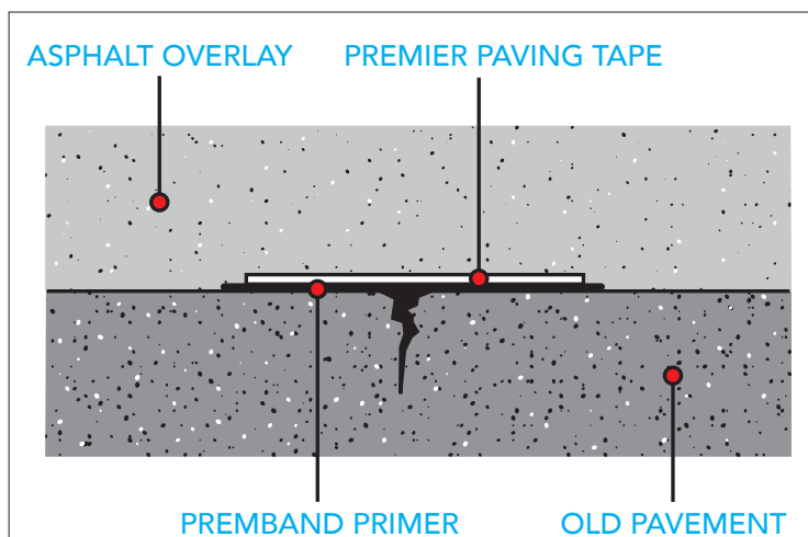
RE-INSTATEMENT TAPE
